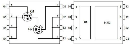
pin assignment
